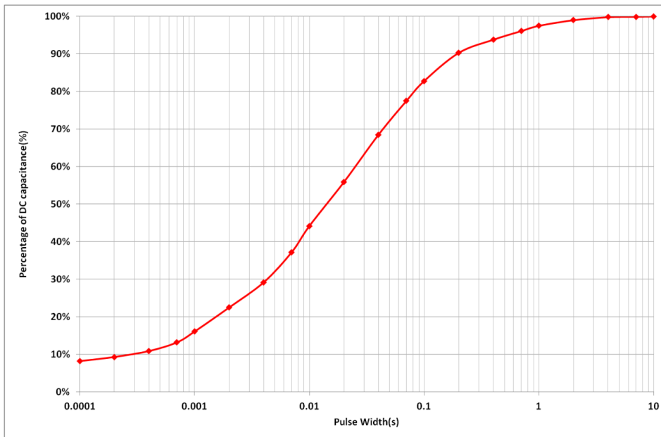
Fig 4: Effective Capacitance
