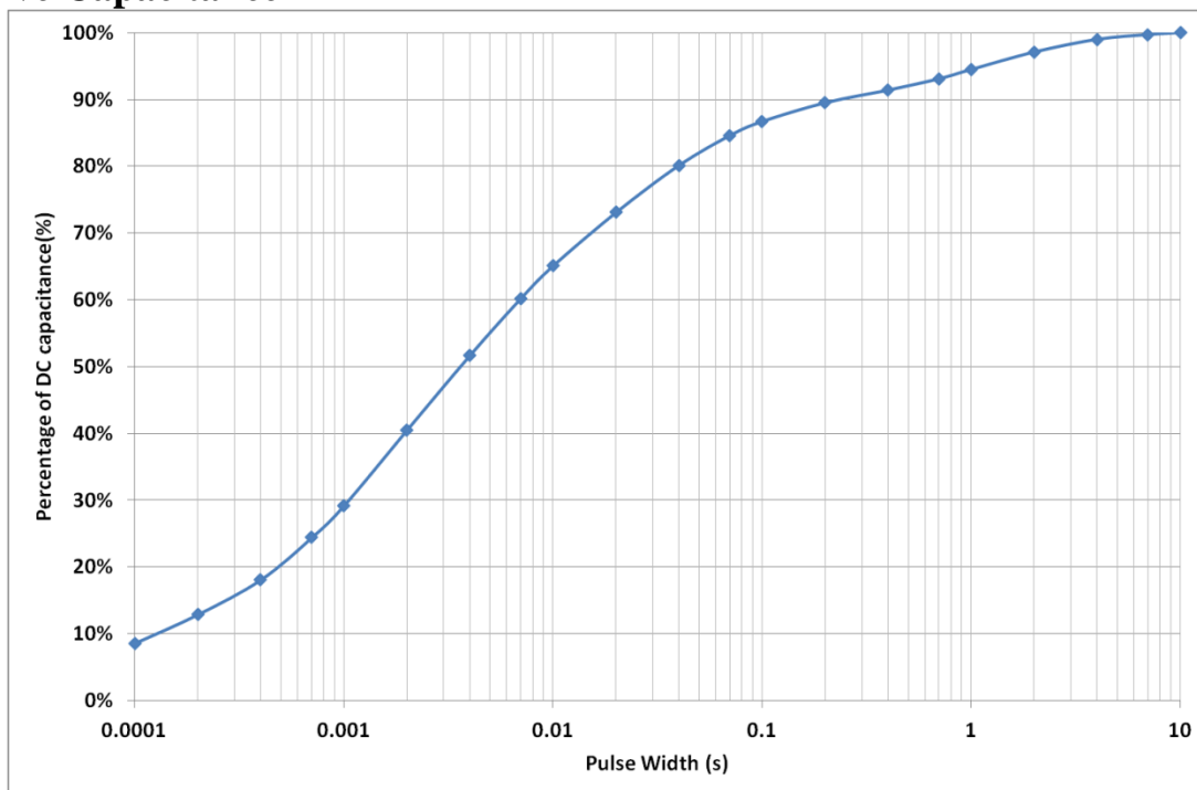
Figure 4: Effective Capacitance
