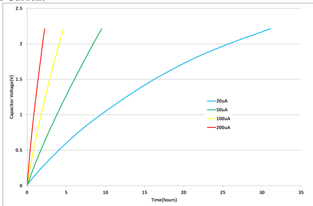
Fig 11: Charging a GS103 with low current
